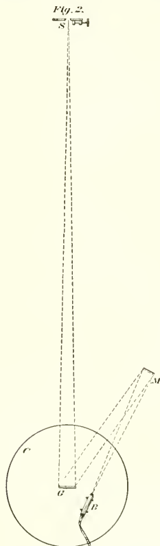
Arrangement of Apparatus for Measuring Angular Direction of a Ray of Heat.
