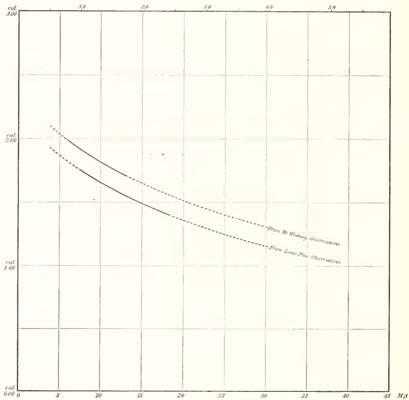
Actinometer Reading as a Function of the "Air Mass."
