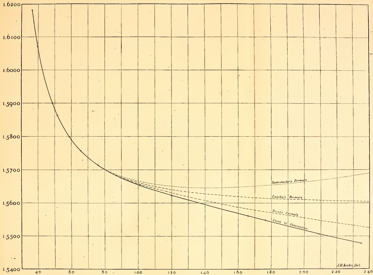
CURVE n-f(\lambda) FOR THE HILGER PRISM.
