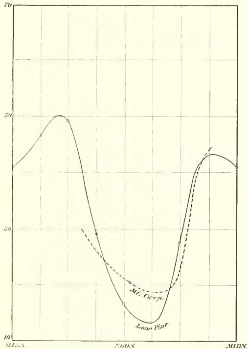
Diurnal Variation of Relative Humidity.
