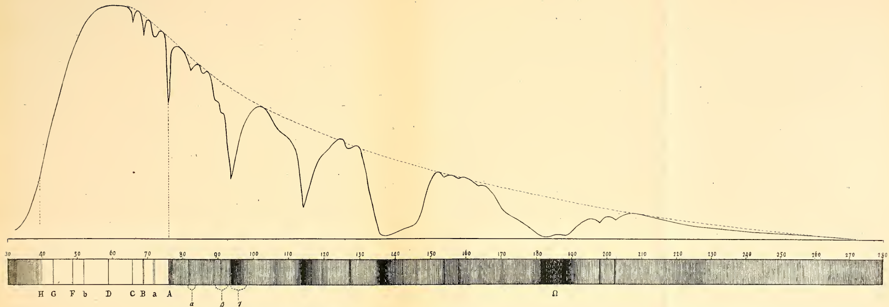
PLATE XII. NORMAL SPECTRUM. (ENERGY CURVE)
