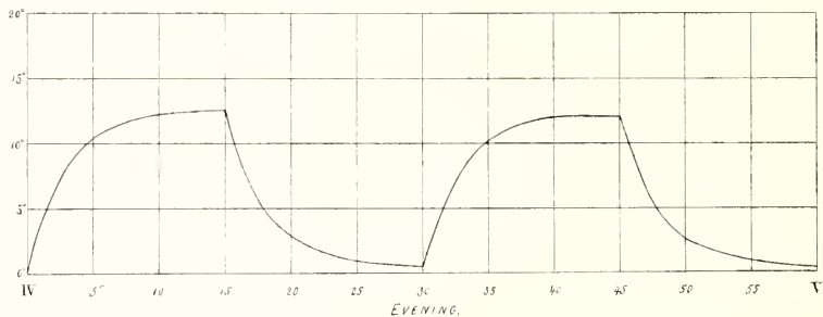
PLATE III ACTINOMETER CURVES FOR AUGUST 4TH, 1881 LONE PINE—ACTINOMETER No. 1.
