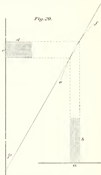
Illustrating Principle of Transformation from the Prismatic to the Normal Spectrum.
