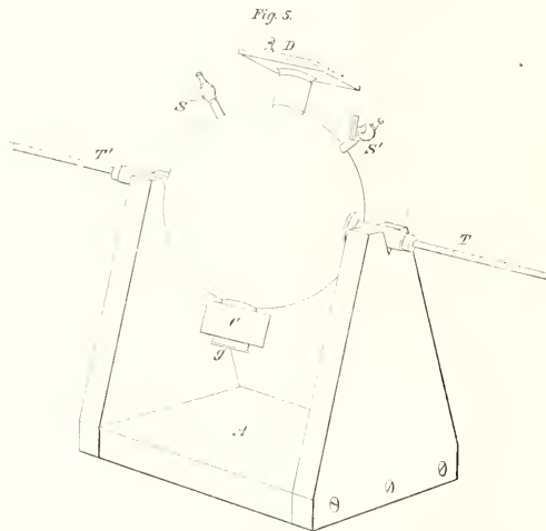
Small Actinometer.—Exterior.
