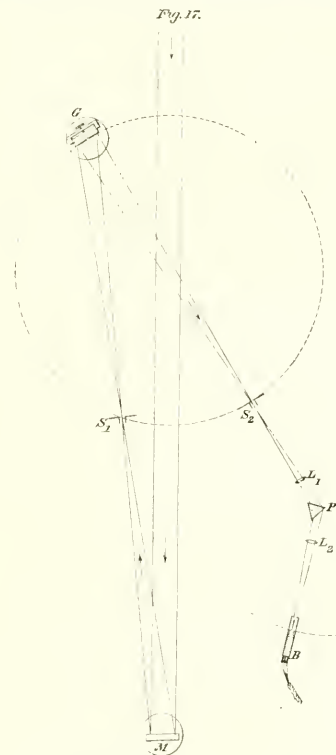
Course of Rays through Apparatus in the determination of lengths of waves of Obscure Heat.
