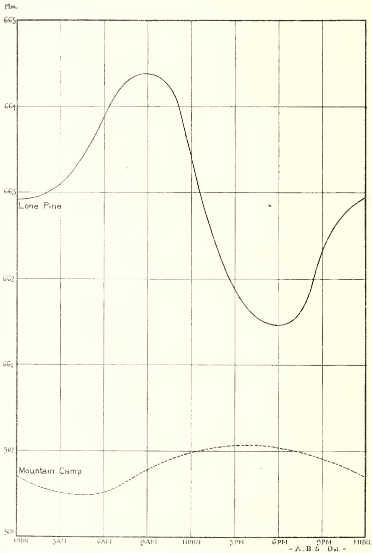
PLATE XVIII. DIURNAL VARIATION OF THE BAROMETER.
