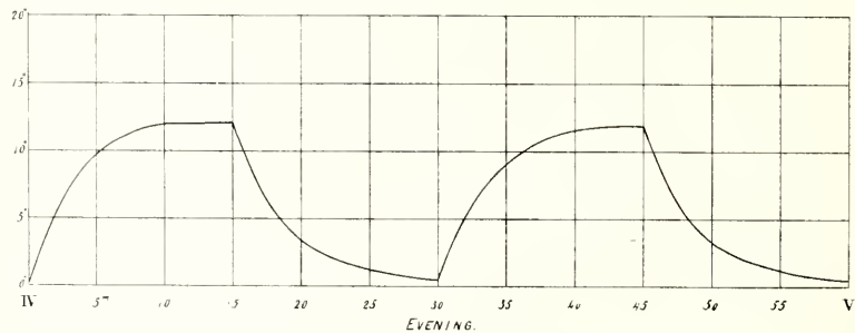
PLATE V. ACTINOMETER CURVES FOR AUGUST 4TH, 1881. LONE PINE—ACTINOMETER NO.3.
