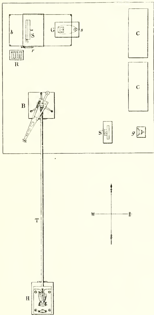
PLATE XIII. PLAN OF TENT AND ARRANGEMENT OF APPARATUS.
