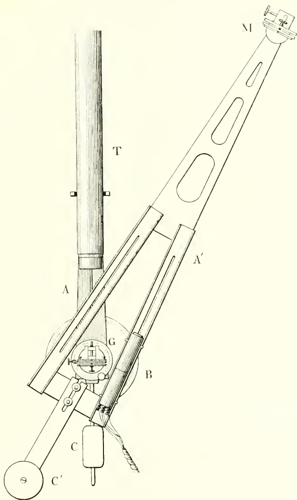
PLATE X SPECTRO-BOLOMETER (PLAN) AS USED FOR MAPPING NORMAL SPECTRUM.
