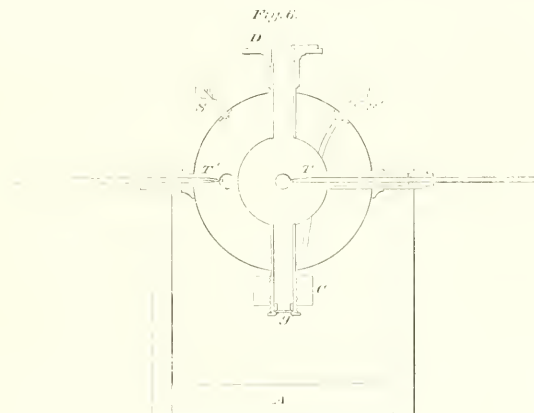
Small Actinometer.—Interior.
