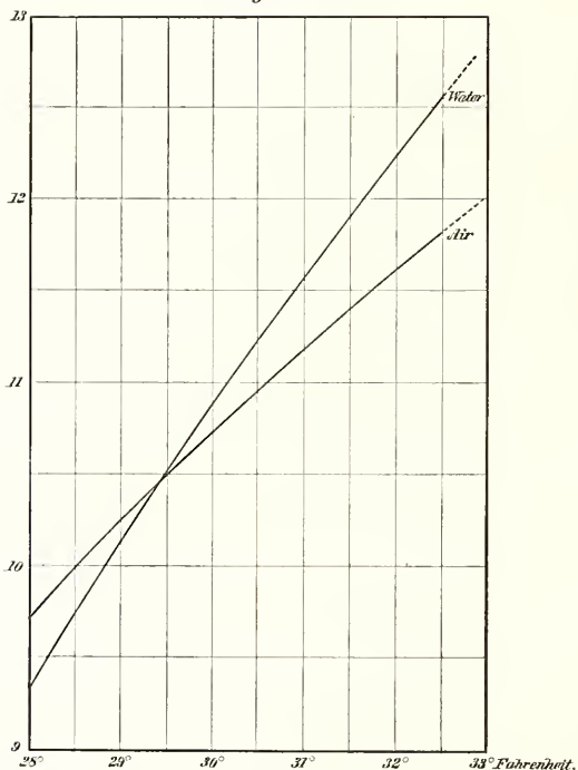
Determination of Mercury in Thermometer, Green, No. 4571.
